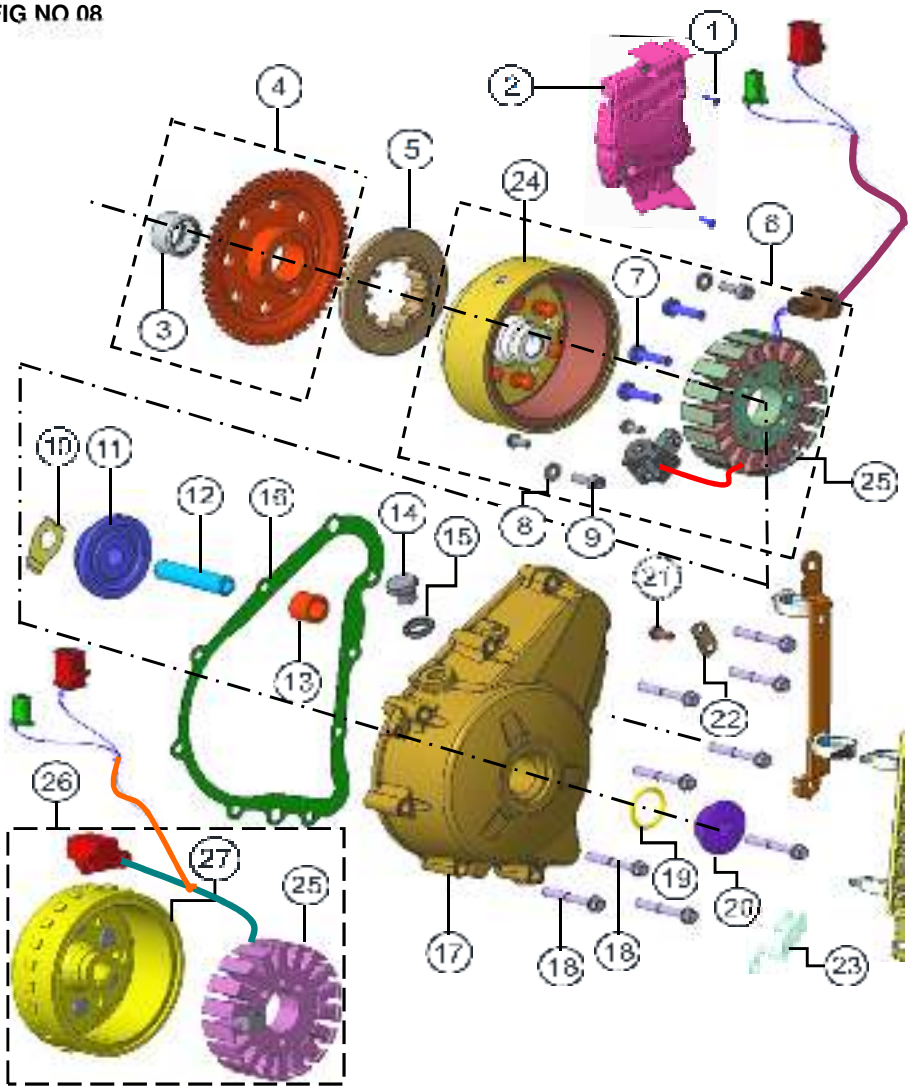
MAGNETO ASSEMBLY
