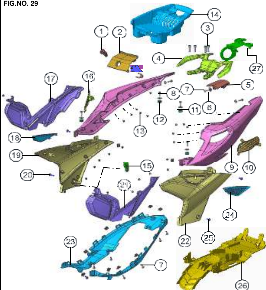
PANEL LH, RH ASSEMBLY
