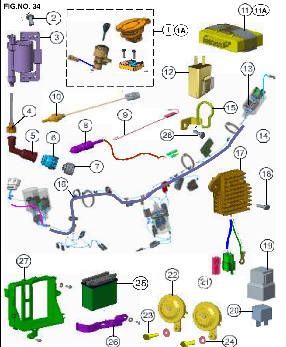
WIRING HARNESS &amp; BATTERY ASSY.
