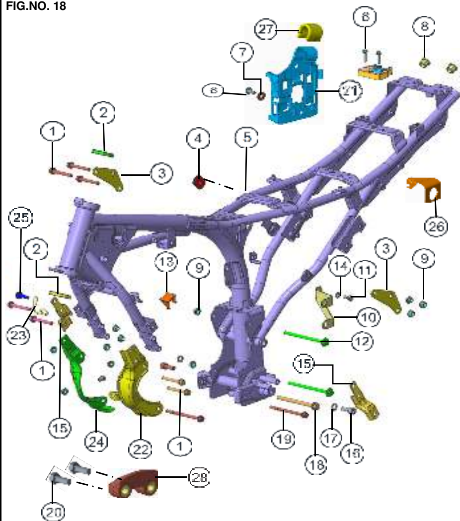
FRAME ASSEMBLY
