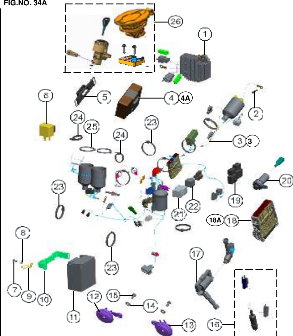
WIRING HARNESS &amp; BATTERY ASSY. EFI
